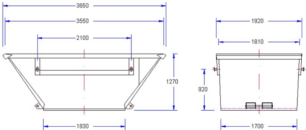
6m 3 Bin Dimensions
