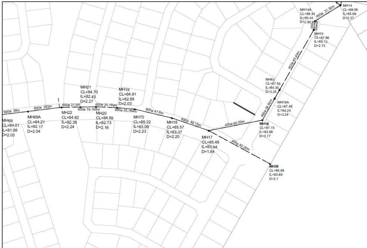
Figure 4: The rising main is to be connected at MH39.
