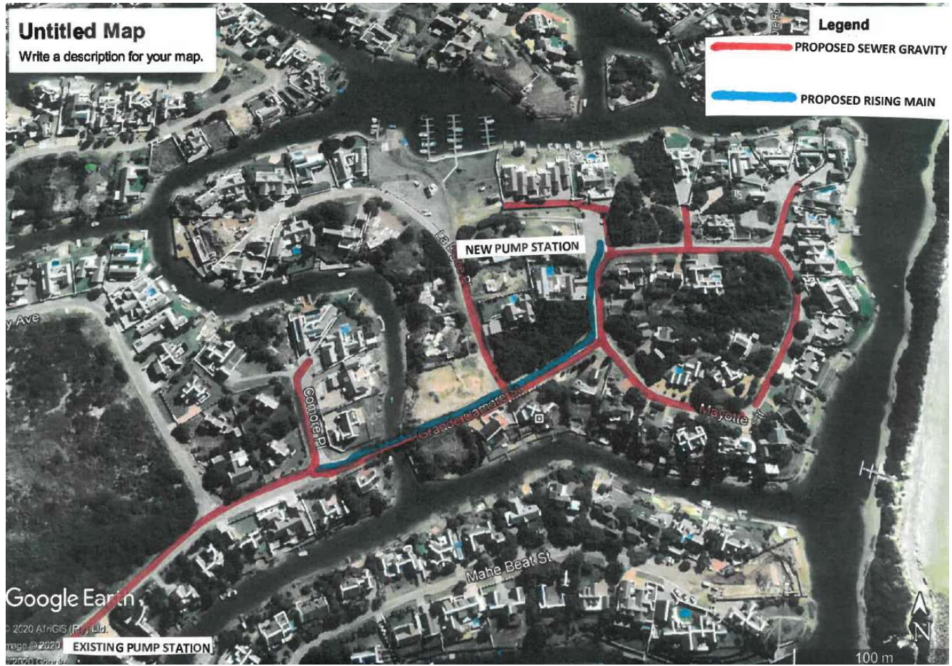
Figure 3: Proposed sewer reticulation network.
