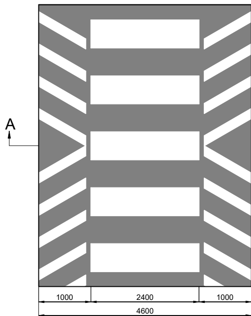
PLAN VIEW ASPHALT
