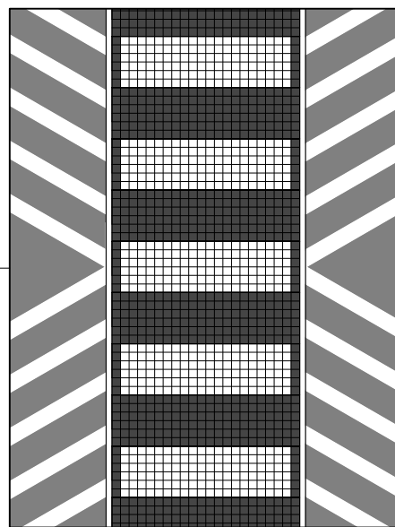
PLAN VIEW BLACK/WHITE FIG 11 EDGE STRIP COBBLES
