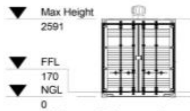
West Elevation 1 : 100
