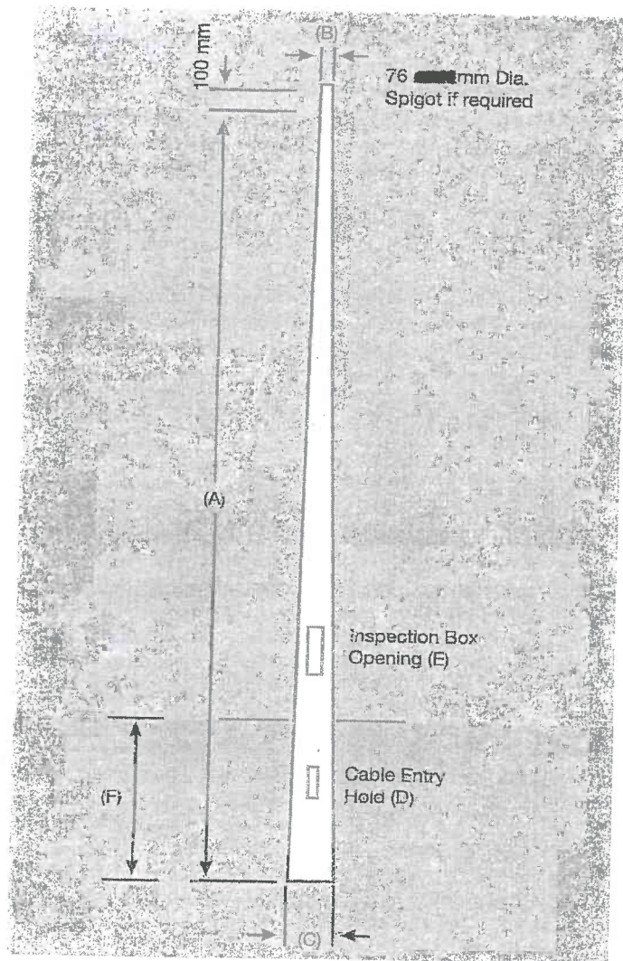
Streetlight Poles - 11m
