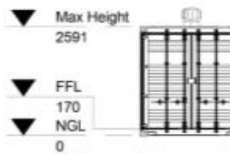
West Elevation 1 : 100
