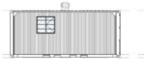
North Elevation 1 : 100
