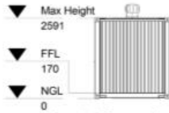
East Elevation 1 : 100
